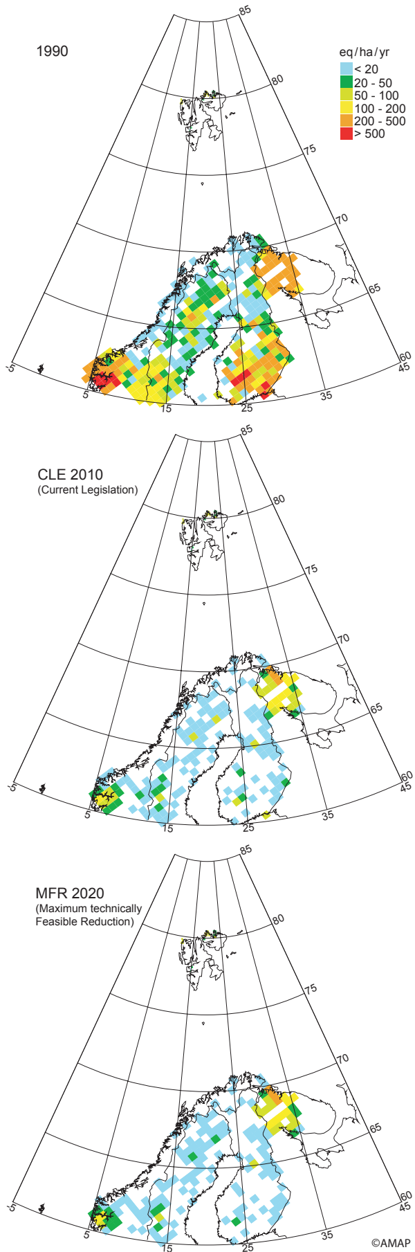
Estimated exceedance of CL_{AC} for surface waters
