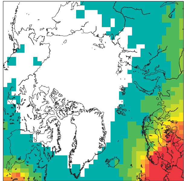
NO 3 deposition in 2000, mg/m 2 /yr
