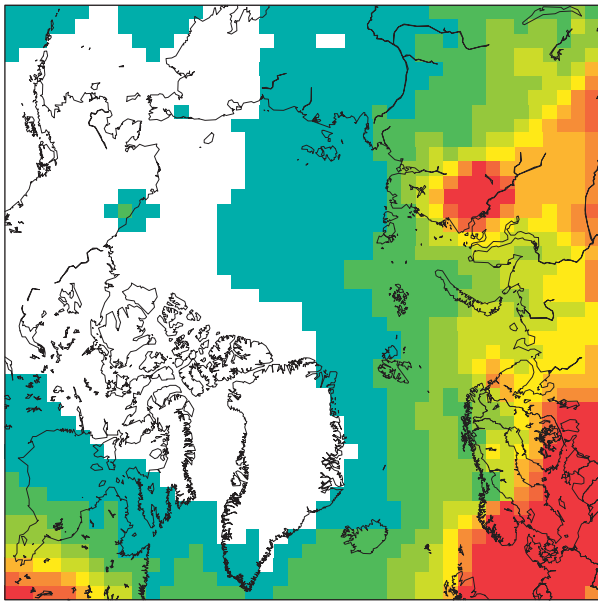
SO x deposition in 2000, mg/m 2 /yr
