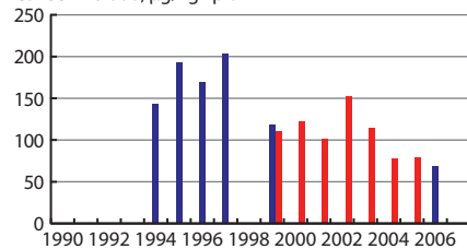
CB153 in blood, \mu\text{g}/\text{kg} lipid
