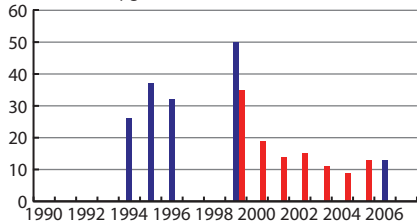
Lead in blood, \mu\text{g}/\text{L}
