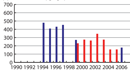
Mercury in blood, \mu\text{g}/\text{L}
