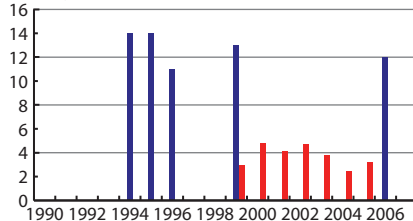
Mercury in blood, \mu\text{g}/\text{L}
