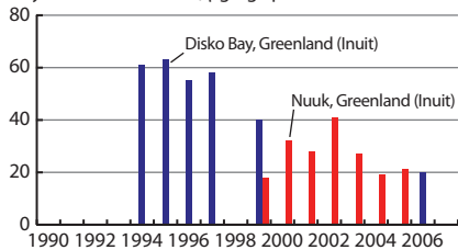
Lead in blood, \mu\text{g}/\text{L}
